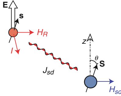
Fig. 4.24 Microscopic origin of the s - d -mediated Rashba field H_R and experimental geometry. Conduction electrons moving perpendicular to E have their spin ( s ) tilted by the Rashba magnetic field ( H_R ), exerting a torque on the localized moments ( S ) through the exchange coupling ( J_{sd} ) and s - d -mediated Rashba field ( H_{Rsd} )
