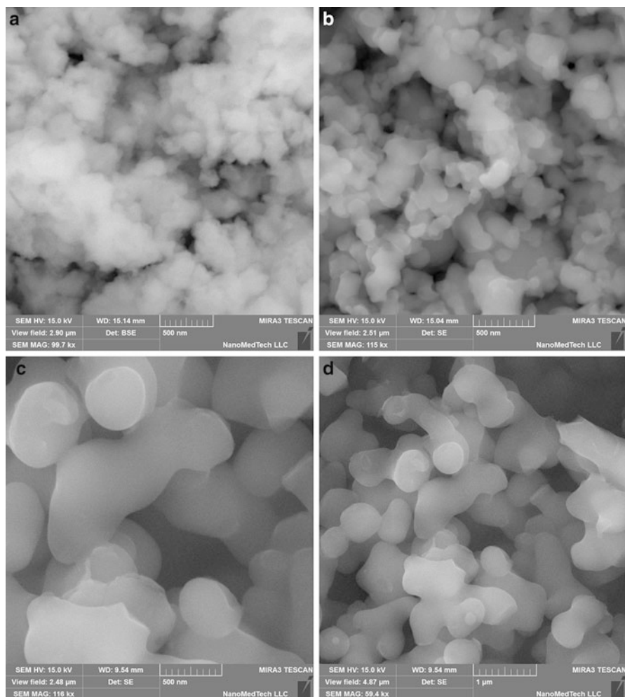
Fig. 30.7 SEM microphoto of powders. (a) \text{Pr(mphpd)}_3 \cdot 2\text{H}_2\text{O} , (b) [\text{Pr(mphpd)}_3]_n , (c) \text{Pr(mphpd)}_3 -co-styrene, scale 500 nm (a–c), 1 μm (d)
