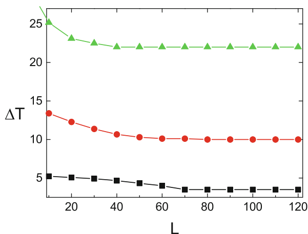
Fig. 10.9 The variation of the thermal hysteresis width for fixed values of fluctuation intensity: \varepsilon = 100 (bottom curve); \varepsilon = 150 (central curve); and \varepsilon = 200 (top curve). The other parameters are those from Fig. 10.7
