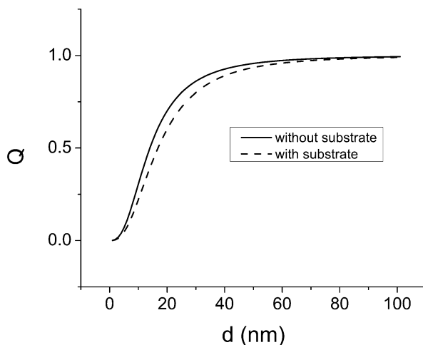
Fig. 27.6 Fluorophore molecule ( q^0 = 1 ) quantum yield Q depending on the distance to the surface of the spherical gold nanoparticle with a radius of 40 nm in the absence (solid line) and in the presence (dashed line) of the glass substrate with \epsilon_2 = 2.59 . d is the distance from the molecule to the nanoparticle surface
