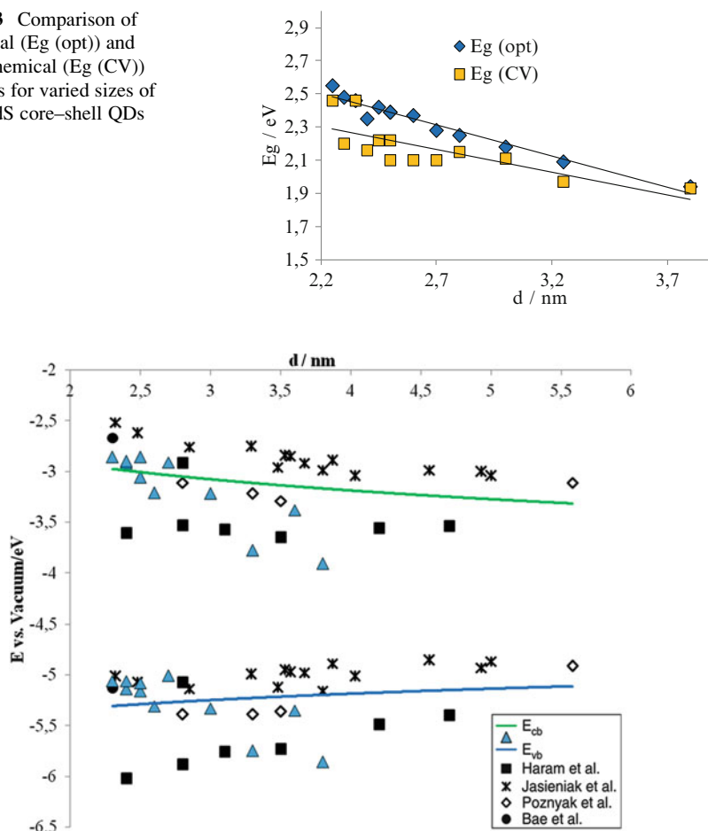
Fig. 17.4 Plot of valence (blue line) and conduction (green line) band edge positions for CdTe/CdS QDs, obtained as a function of size from the respective anodic (A) and cathodic (C) peaks (blue triangles)
