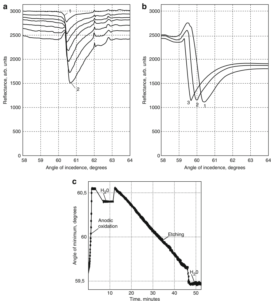
Fig. 29.4 Monitoring of formation of sensor structures Al/porous \text{Al}_2\text{O}_3 by the Plasmon test device. (a) Change in the shape of the reflection curve in the process of anodic oxidation of aluminum film on glass for MCWG Al/porous \text{Al}_2\text{O}_3 fabrication: 1, appearance of waveguide mode; 2, final of anodic oxidation. (b) Change in the shape of the reflection curve in the etching process: 1, beginning of the etching; 3, final structure. (c) Sensogram received during the process of formation of MCWG structure Al/porous \text{Al}_2\text{O}_3
