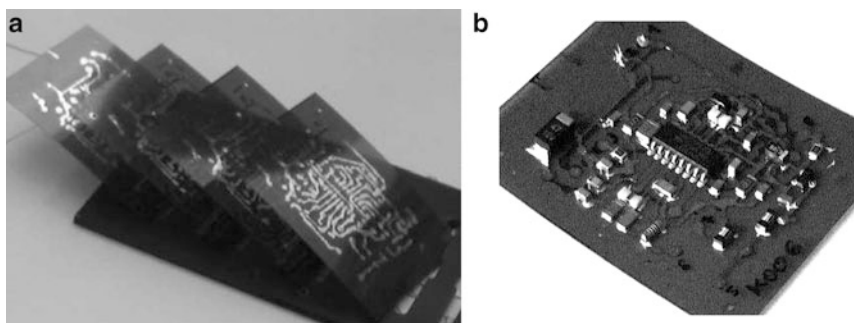
Fig. 31.1 (a) Polyimide substrates ( 40 \times 50 mm) with printed silver conductive tracks after thermal sintering by 250^\circ\text{C} for 60 min. Specific conductivity of patterns \approx 2 \times 10^7 S/m. (b) VHF radio after surface mounting of components with conductive glue [1]
