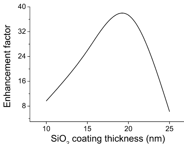
Fig. 27.11 Dependence of the fluorescence enhancement factor of R6G dye on the thickness of the \text{SiO}_2 dielectric coating on the gold nanostructures
