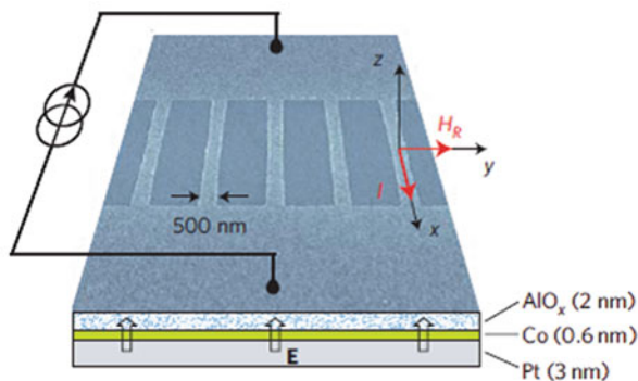
Fig. 4.25 Scanning electron micrograph detail of the magnetic nanostructure Pt/Co/AlO x wire array and schematic vertical cross section of the layer. Arrows indicates the direction of the current ( I ), interfacial electric field ( E||z ), and H_R . The sign of E is determined from the measured orientation of I and H_{Rsd} assuming positive polarization of the conduction electrons near the Fermi level
