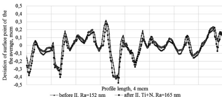
Fig. 12.2 Profiles of surface texture of standards before and after ionic implantation (II)
