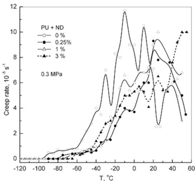
Fig. 9.7 Creep rate spectra obtained for neat PU network and ND-containing nanocomposites based thereon at tensile stress of 0.3 MPa in the temperature region of glass transition. ND weight contents are indicated [22]
