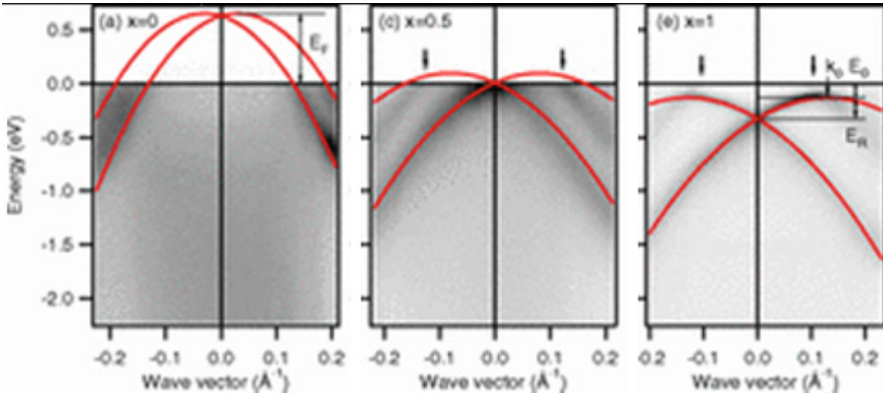
Fig. 4.23 Experimental band structures of \text{Bi}_x\text{Pb}_{1-x}/\text{Ag}(111) surface alloys for x , obtained by angle-resolved photoelectron spectroscopy, where k_0 is the spin–orbit splitting and E_R is the Rashba energy
