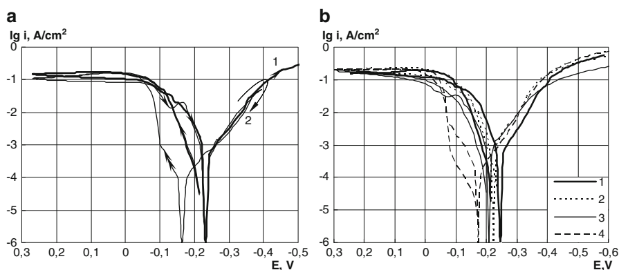
Fig. 7.1 Anode-cathodic polarization curves for steel electrode in (a) 1—0.5 M \text{H}_2\text{SO}_4 ; 2—0.5 M \text{H}_2\text{SO}_4 + 1 g/L DPA (circular polarization) (b) 1—0.5 M \text{H}_2\text{SO}_4 ; 2—0.5 M \text{H}_2\text{SO}_4 + 1 g/L DPA; 3—0.5 M \text{H}_2\text{SO}_4 + 1 g/L DPA + 2 g/L \text{Fe}_2(\text{SO}_4)_3 ; 4—0.5 M \text{H}_2\text{SO}_4 + 1 g/L DPA + 2 g/L \text{Fe}_2(\text{SO}_4)_3 + 2 g/L KI
