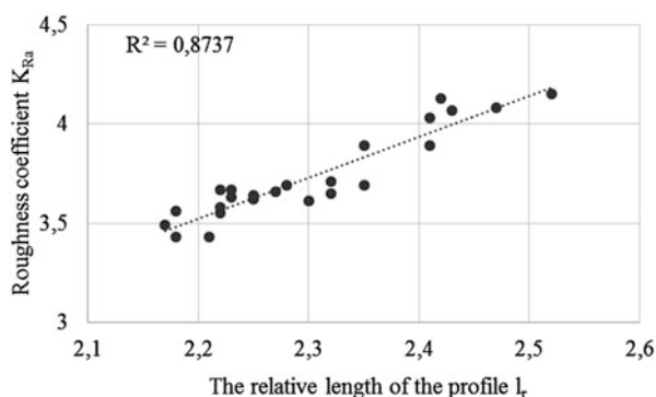
Fig. 12.3 Dependence of coefficient of roughness on relative length of profile
