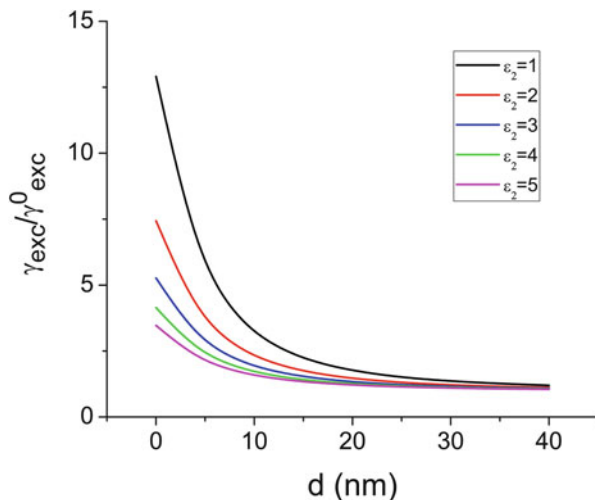
Fig. 27.5 Fluorophore molecule excitation rate change near the spherical gold nanoparticle with a radius of 20 nm for different values of the substrate dielectric permittivity. \epsilon_2 is the substrate dielectric permittivity, d is the distance from nanoparticle surface to the point of fluorophore molecule location
