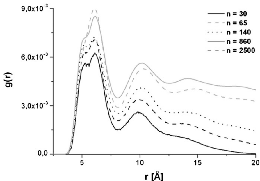
Fig. 25.5 The comparison of the radial distribution function of homocysteine for all studied systems, at T = 290 K
