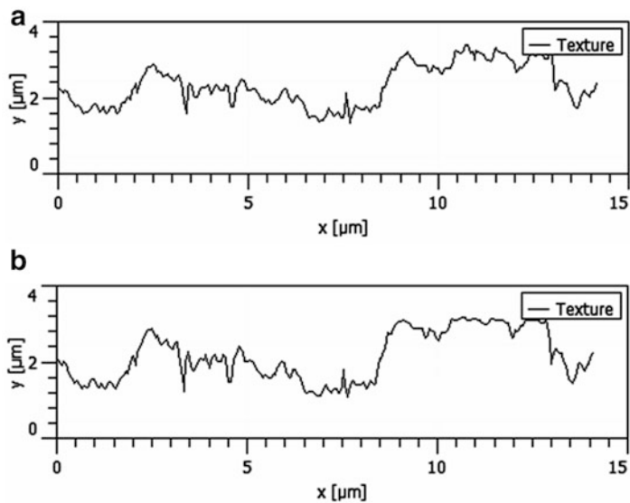
Fig. 12.5 Profiles of standards: (a) Ti/SS; (b) Ti/SS, modeled by neural network
