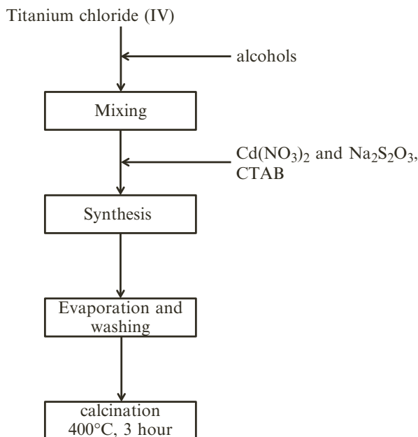
Fig. 19.7 Scheme of synthesis of \text{TiO}_2 particles from \text{TiCl}_4
