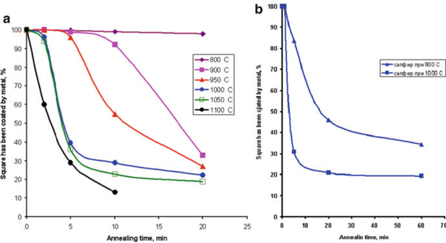
Fig. 3.5 Dependence of sapphire square coated by metallic film from annealing time under various temperature (800–1,100 °C): (a) copper; (b) aurum
