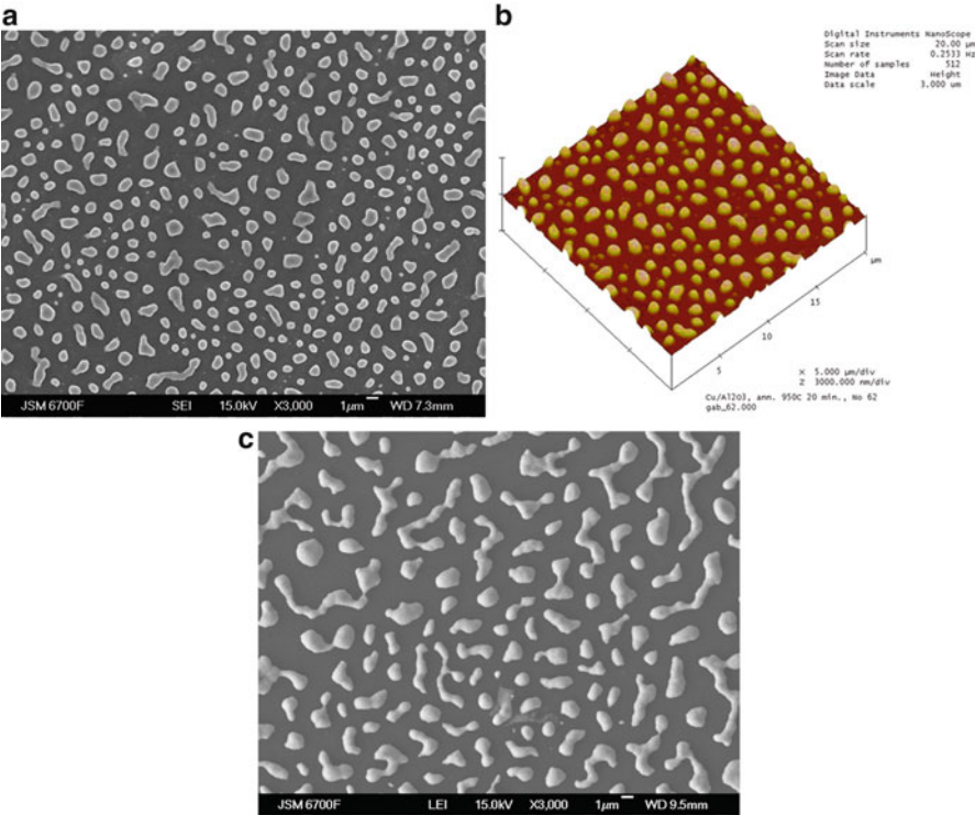
Fig. 3.4 Copper film 100 nm thickness deposited onto sapphire and annealed in vacuum has been investigated using scanning microscopy (a, c) \times 3,000 and atomic force microscopy (b): (a, b) 950^{\circ}\text{C} , 20 min; (c) 1,000^{\circ}\text{C} , 5 min
