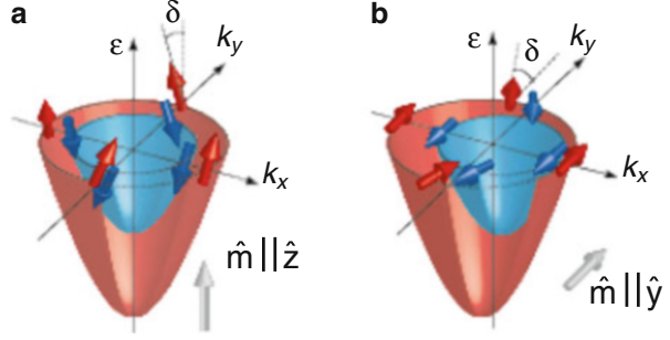
Fig. 4.29 Two Fermi sheets of conduction electrons created by the Rashba spin–orbit splitting in magnetic metals with different directions of the magnetization \mathbf{m} : (a) \mathbf{m} \parallel \hat{z} , (b) \mathbf{m} \parallel \hat{y}
