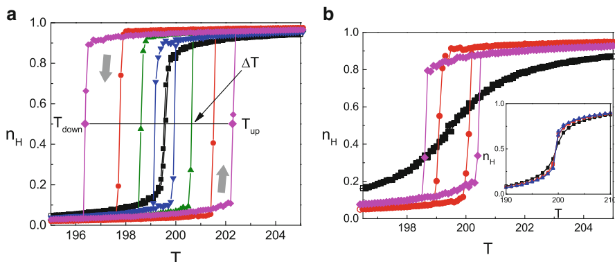
Fig. 10.10 The spin transition curves for different statistical characteristics of fluctuations for J = 85 (a) and J = 70 (b). The curve marked by squares (black online) corresponds to fluctuationless system; marked by circles (red online) corresponds to white uncorrelated fluctuations; marked by triangles up (green online) is for C = 0 and \tau = 2.5 ; marked by triangles down (blue online) is for C = 0 and \tau = 5 ; marked by diamonds (pink online) is for C = 0.5 and \tau = 5 . Here the system size is 70 \times 70 . In the inset of (b) one presents the transition curves for fixed white noise intensities \epsilon = 100 [black (squared) line]; \epsilon = 115 [red (circled) line], and \epsilon = 120 [blue (triangled) line] for J = 50
