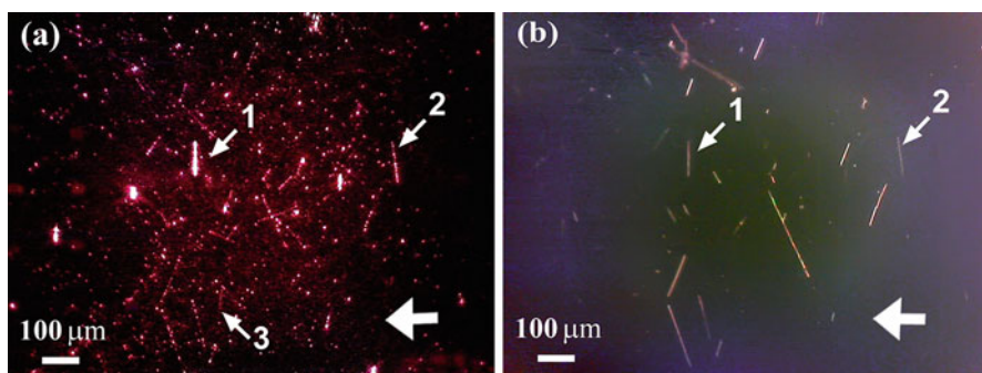
Fig. 20.2 Images of Si-rods in the SPR-enhanced TIRM (a), image of the same area obtained using standard light microscope under directional illumination (b). Correspondent details are indicated with numbered arrows . There is no visible counterpart for the rod 3 under directional light. Bold arrows indicate the illumination direction
